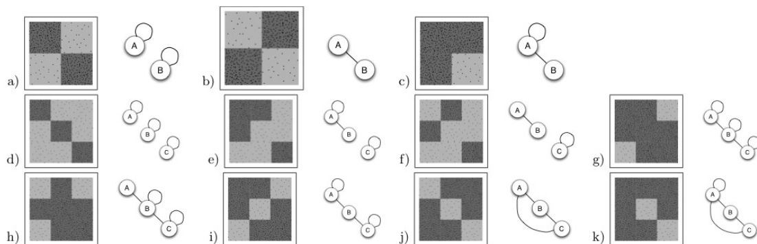
Fig.1. Example adjacency matrices and corresponding image graphs with two and three roles. Nodes with the same pattern of connectivity appear as blocks in the adjacency matrix and are represented by a single node in the image graph. Background shading of matrices reflects link density in blocks. We show only those three role models which are not isomorphic and which cannot be reduced to a block model of two roles only. The two-role-models can be understood as a) modular structure, where nodes connect primarily to nodes of the same role, b) bipartition, with connections primarily between nodes of different type and c) a core-periphery structure with nodes of type A (the core) connecting preferentially among themselves and to nodes of type B (the periphery). The three role models can be seen as combinations of these three basic structures plus the possibility of having intermediates.
